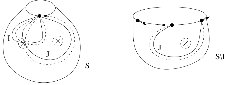
Figure 1: 1-sided arcs
