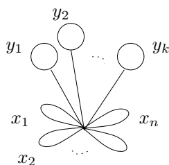
Figure 1: G_{n,k}
