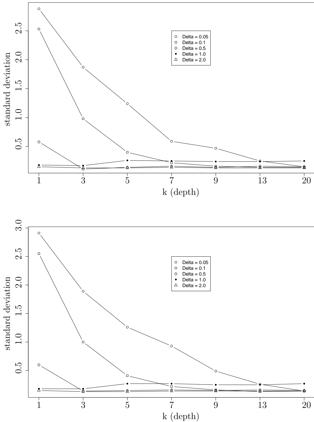
Figure 6.2: Standard deviation of the pseudo-likelihood estimator of a (upper) and b (lower) for various values of the the depth k and the time between observations \Delta . The number of observations is 200, and the true parameter values are a = -1 and b = 0.95 .
