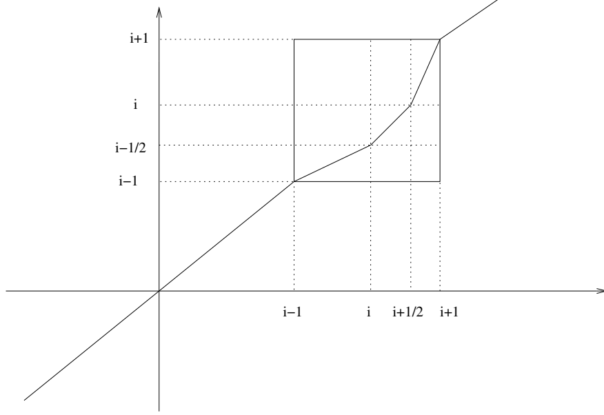
FIGURE 4. Graph of \tilde{G}_i = y_i y_{i+1}^{-1} , i \in \mathbb{Z}
