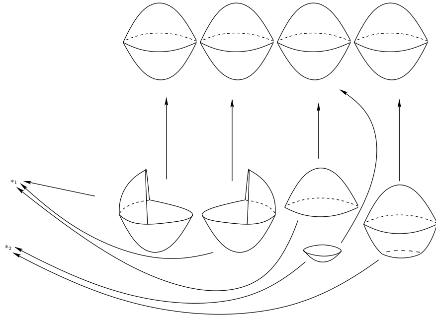
Figure 1.6: The 4-ary operation of the introduction has the complement of its timber \mathcal{CN}_1, \mathcal{CN}_2, \mathcal{CN}_3, \mathcal{CN}_4 drawn as the five disks on the bottom right corner. The upwards arrow are the inclusion maps, so that dualizing them provides the restriction map. The leftwards maps have as target two points, and these should be considered as collapsing the components of the blueprint \beta_{[T, P_1, P_2, P_3]} . These maps are given as the ones where the boundary of each disk is contained in a component of the blueprint.
