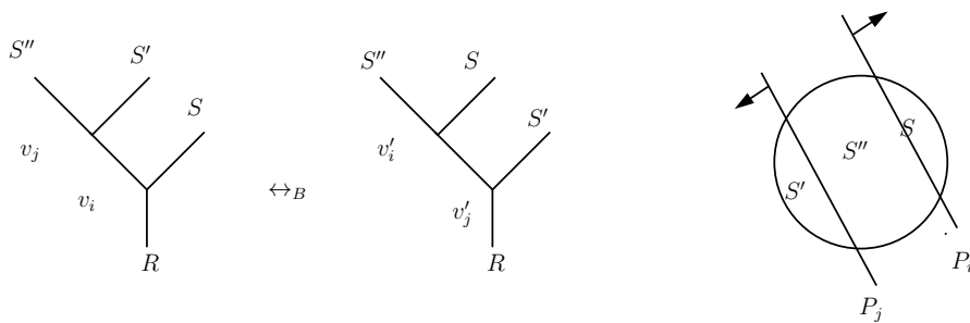
Figure 1.4: The \leftrightarrow_B -relation
