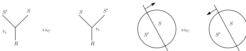
Figure 1.3: The \leftrightarrow_C -relation
