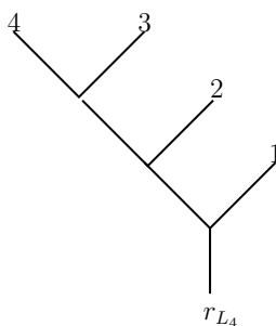
Figure 1.5: The left-blown tree L_4
